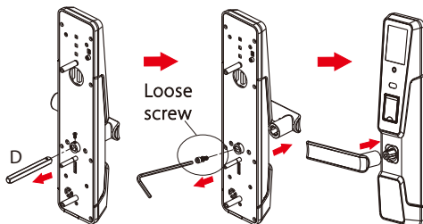
Front Lock
